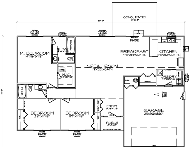
FIRST FLOOR PLAN A-3
