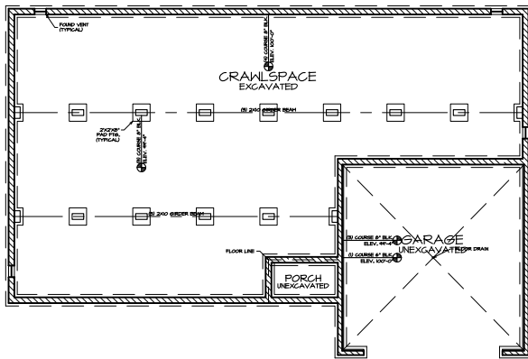
FOUNDATION PLAN A-2
